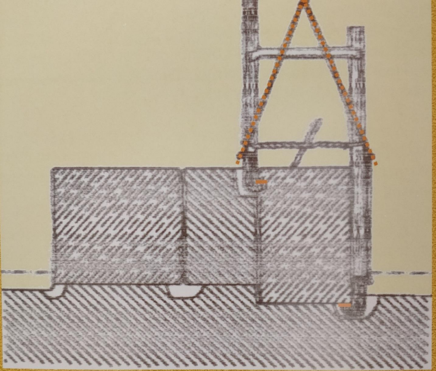
CLAW-LIFT, OFF-SET, PLACING BLOCKS ADJACENT.
